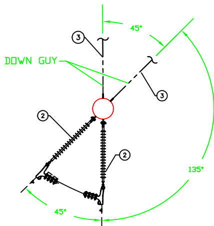
OVERHEAD VIEW
