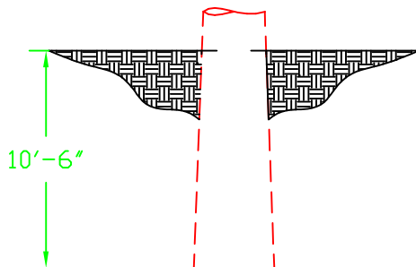
85' STRUCTURE EMBEDMENT
