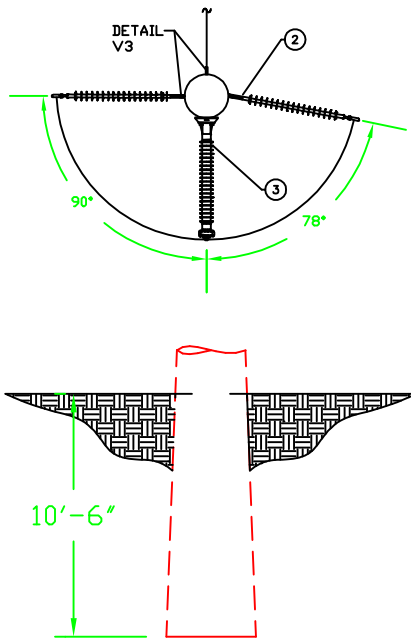
85' Structure Embedment
