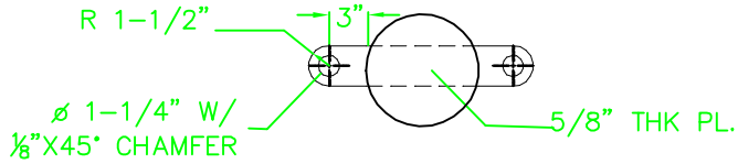
DETAIL V1 HORIZONTAL OHGW/DISTRIBUTION VANG
