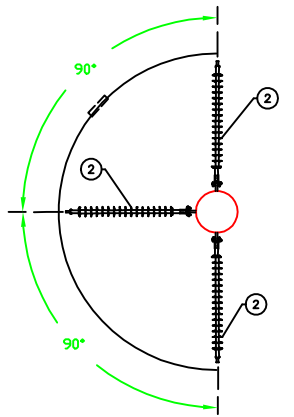
OVERHEAD VIEW
