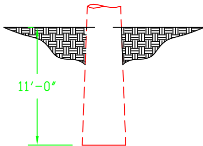
90' Structure Embedment
