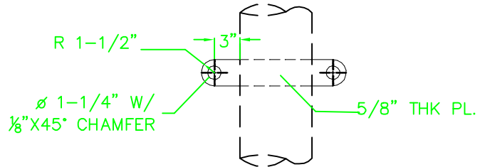
DETAIL V4 VERTICAL OHGW/DISTRIBUTION VANG
