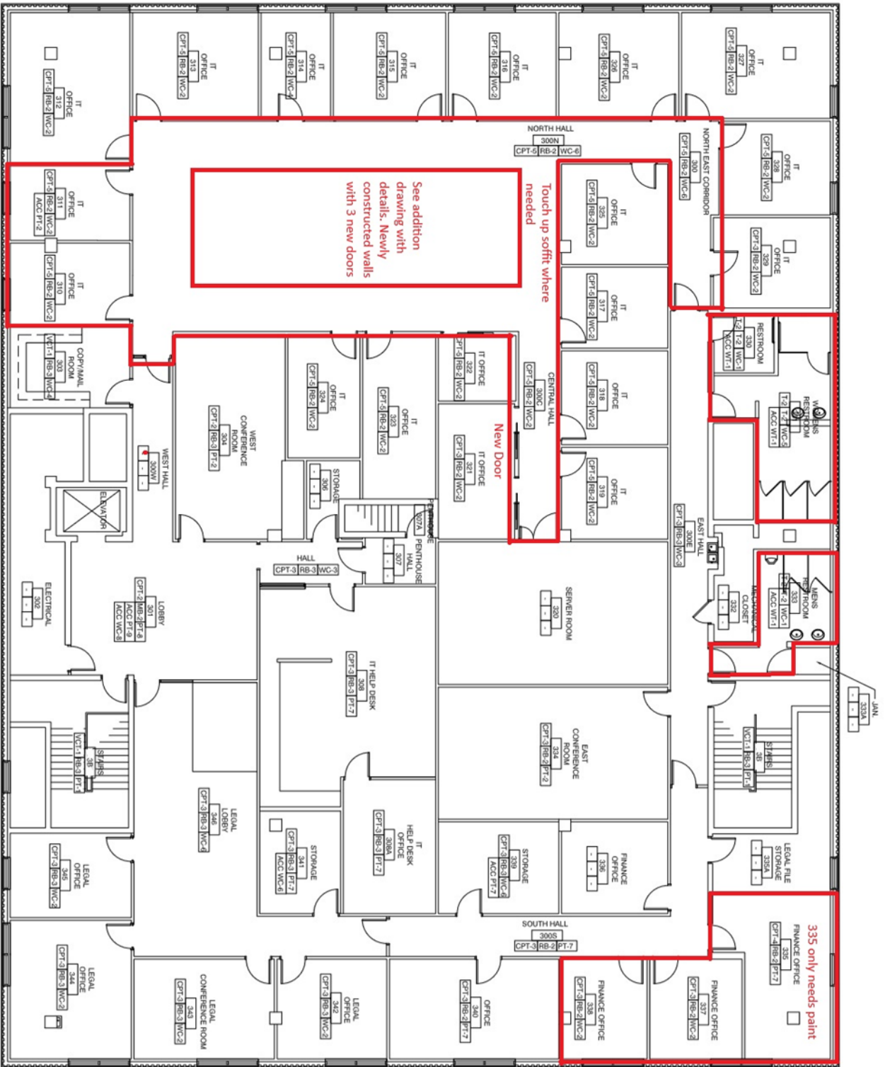
THIRD FLOOR FINISH PLAN 1
