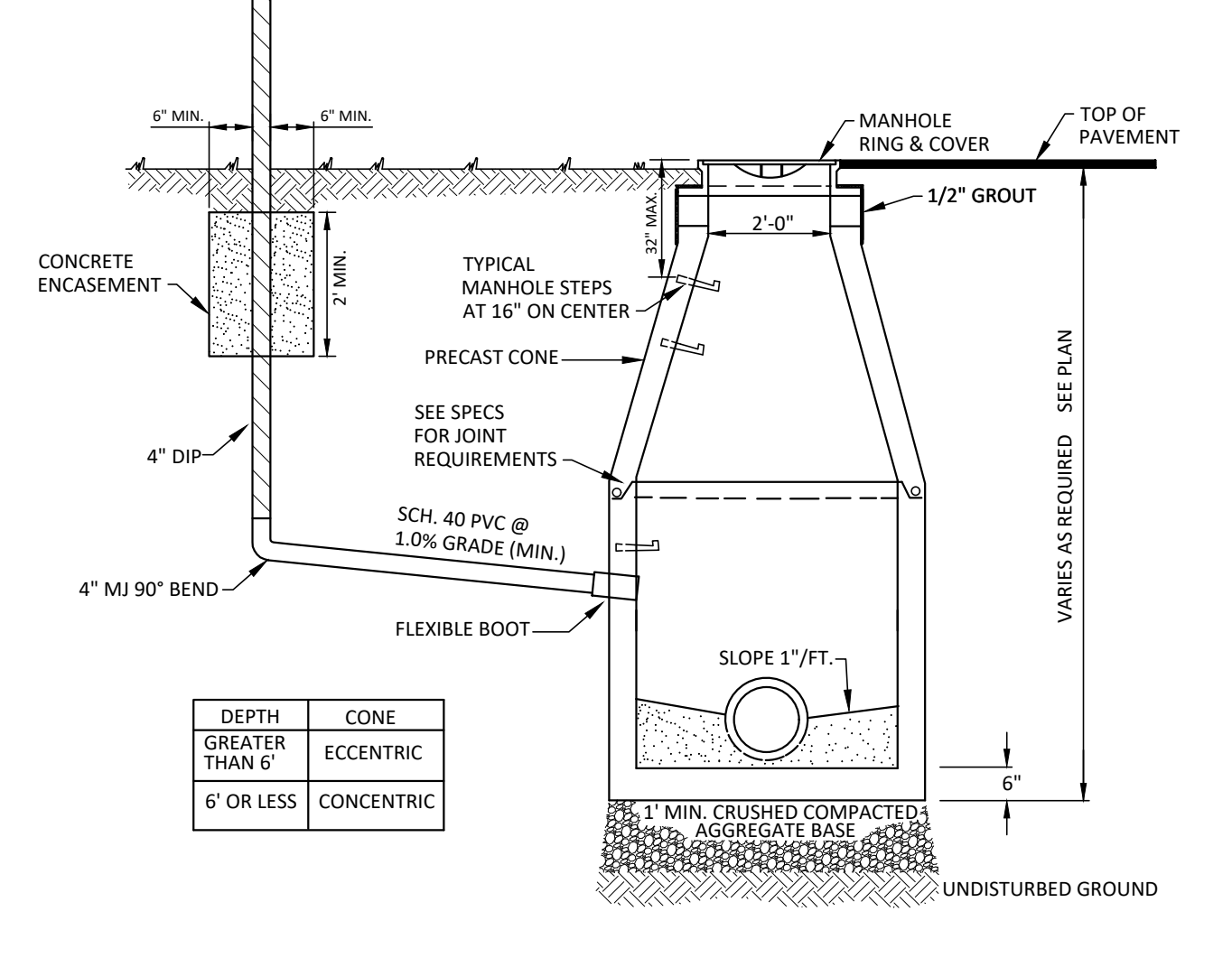
TYPICAL PRECAST VENTED MANHOLE NOT TO SCALE
