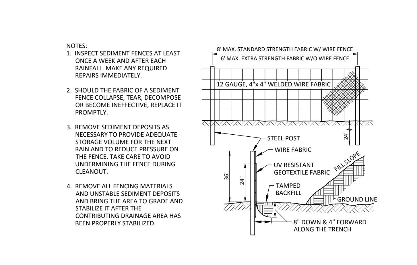
TEMPORARY SILT FENCE NOT TO SCALE
