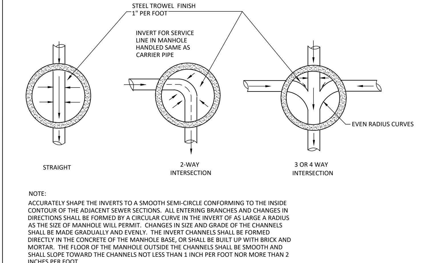
MANHOLE INVERTS (S-17) NOT TO SCALE
