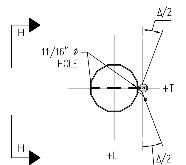
SECTION E-E (N.T.S.) COMMUNICATIONS ATTACHMENT "AT-XXX27DT-144-CLCB" 144 FIBER
