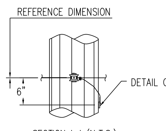
SECTION I-I (N.T.S.) DISTRIBUTION NEUTRAL 1/0 6/1 STRAND "RAVEN" ACSR
