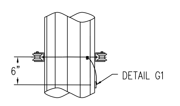
SECTION G-G (N.T.S.) COMMUNICATIONS ATTACHMENT "AT-XXX27DT-144-CLCB" 144 FIBER
