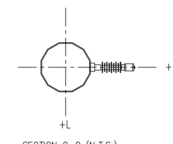
SECTION C-C (N.T.S.) DISTRIBUTION ATTACHMENT 336.4 KCMIL 18/1 STRAND "MERLIN" ACSR
