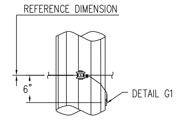
SECTION H-H (N.T.S.) COMMUNICATIONS ATTACHMENT "AT-XXX27DT-144-CLCB" 144 FIBER
