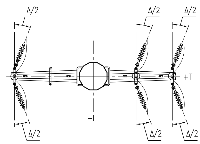
SECTION C-C, D-D (N.T.S.) DISTRIBUTION ATTACHMENT 795 KCMIL 37/0 STRAND 'ARBUTUS' AAC
