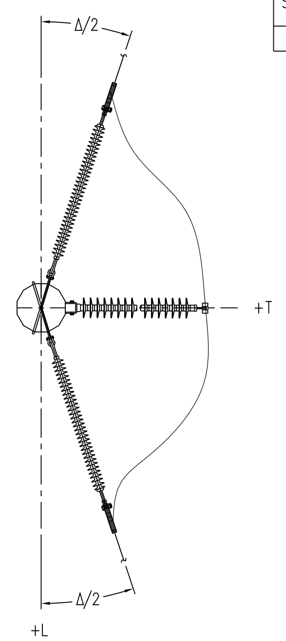
SECTION B-B (N.T.S.) CONDUCTOR ATTACHMENT 1272 KCMIL 61/0 STRAND 'NARCISSUS' AAC
