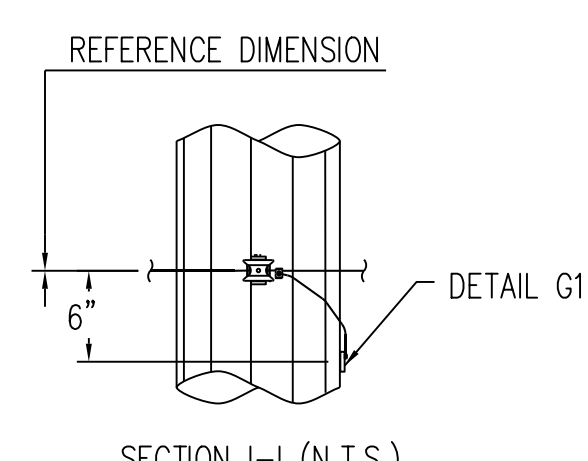
SECTION I-I (N.T.S.) DISTRIBUTION NEUTRAL 336.4 KCMIL 18/1 STRAND "MERLIN" ACSR
