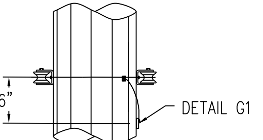
SECTION H-H (N.T.S.) COMMUNICATIONS ATTACHMENT 'AT-XXX27DT-144-CLCB' 144 FIBER
