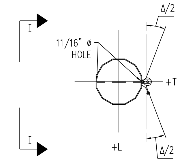
SECTION D-D (N.T.S.) DISTRIBUTION NEUTRAL 1/0 6/1 STRAND "RAVEN" ACSR
