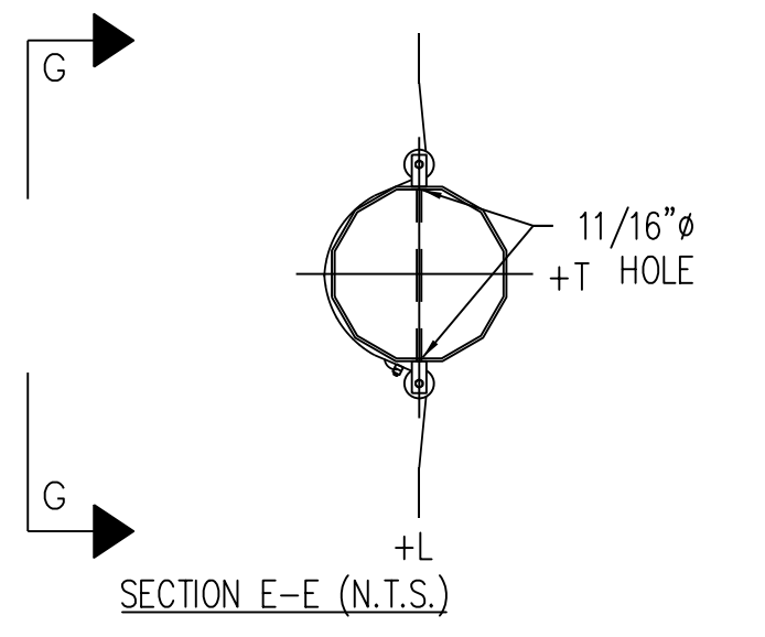
SECTION E-E (N.T.S.) COMMUNICATIONS ATTACHMENT "AT-XXX27DT-144-CLCB" 144 FIBER
