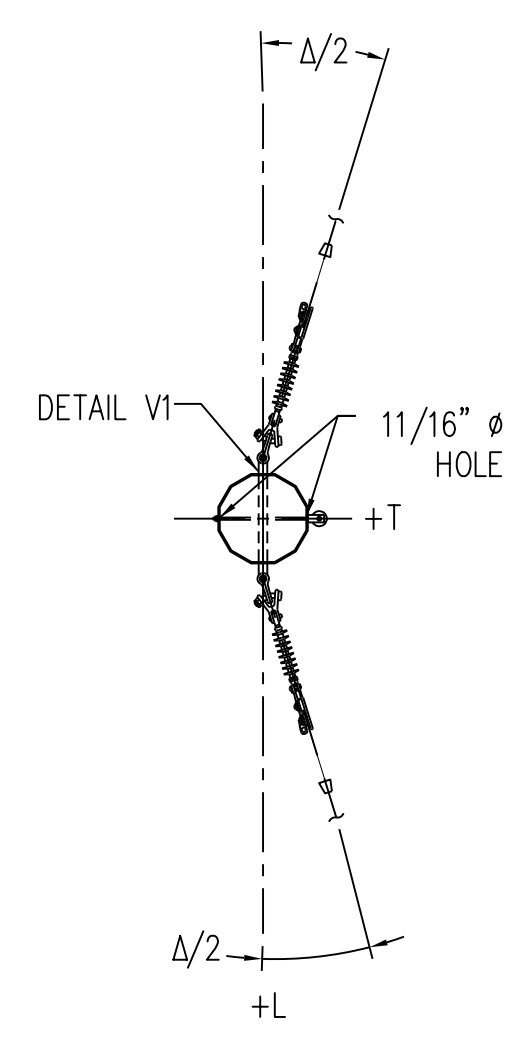
SECTION E-E (N.T.S.) NEUTRAL ATTACHMENT 336.4 KCMIL 18/1 STRAND 'MERLIN' ACSR
