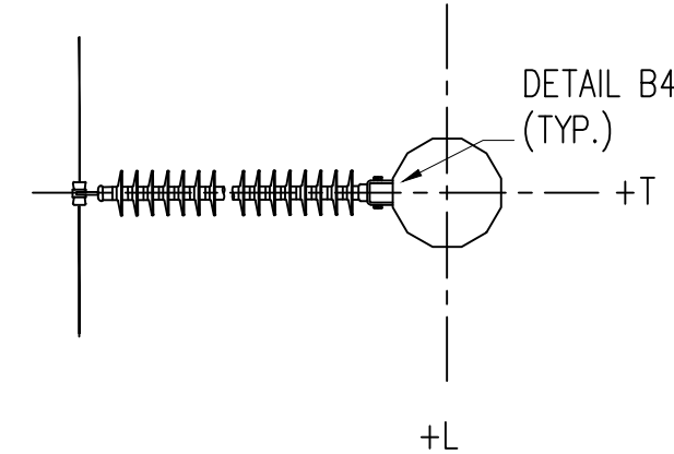
SECTION B-B, D-D (N.T.S.) CONDUCTOR ATTACHMENT 115KV: 1272 KCMIL 61/0 STRAND "NARCISSUS" AAC
