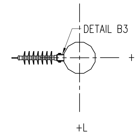
SECTION F-F (N.T.S.) DISTRIBUTION ATTACHMENTS 1/0 ACSR "RAVEN"
