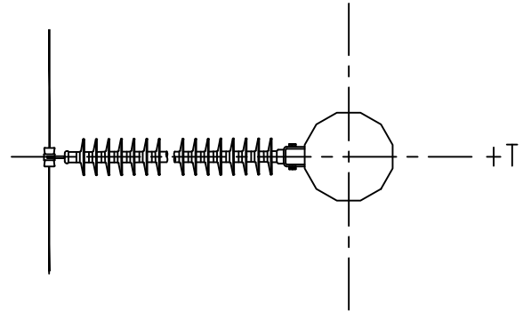
SECTION B-B, D-D (N.T.S.) CONDUCTOR ATTACHMENT 115KV: 1272 KCMIL 61/0 STRAND "NARCISSUS" AAC
