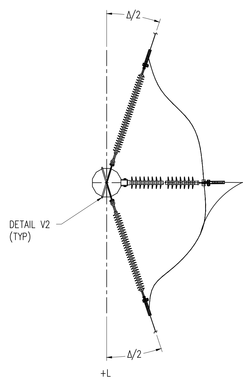
SECTION B-B (N.T.S.) CONDUCTOR ATTACHMENT 1272 KCMIL 61/0 STRAND "NARCISSUS" AAC
