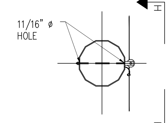
SECTION G-G (N.T.S.) COMMUNICATIONS ATTACHMENT ADSS: "AT-XXX27DT-144-CLCB" 144 FIBER
