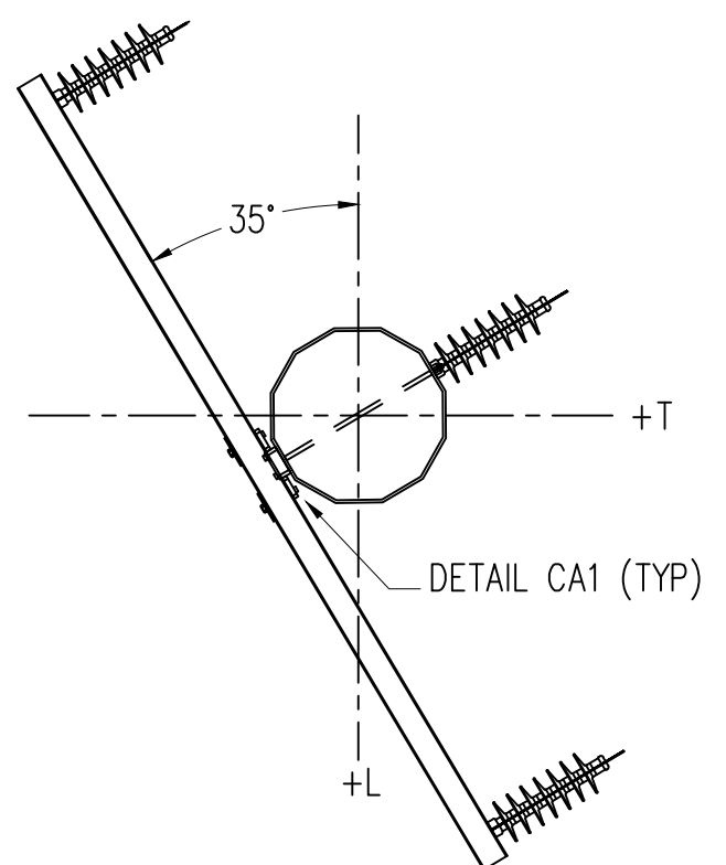
SECTION F-F (N.T.S.) DISTRIBUTION ATTACHMENT 336.4 KCMIL 18/1 STRAND "MERLIN" ACSR
