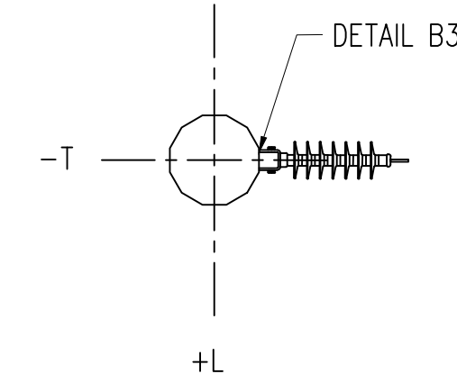
SECTION F-F (N.T.S.) DISTRIBUTION ATTACHMENTS 1/0 ACSR "RAVEN"
