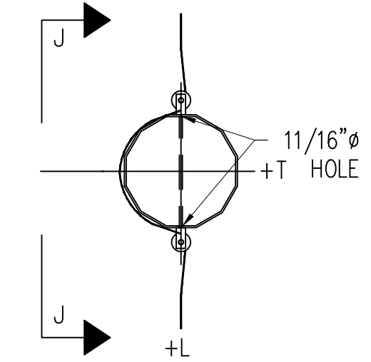
SECTION H-H (N.T.S.) COMMUNICATIONS ATTACHMENT "AT-XXX27DT-144-CLCB" 144 FIBER
