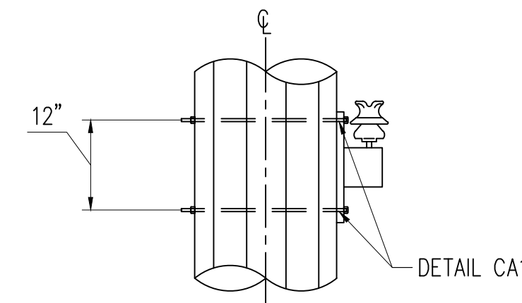
SECTION K-K (N.T.S.) DISTRIBUTION ATTACHMENT, 795 KCMIL AAC "ARBUTUS"
