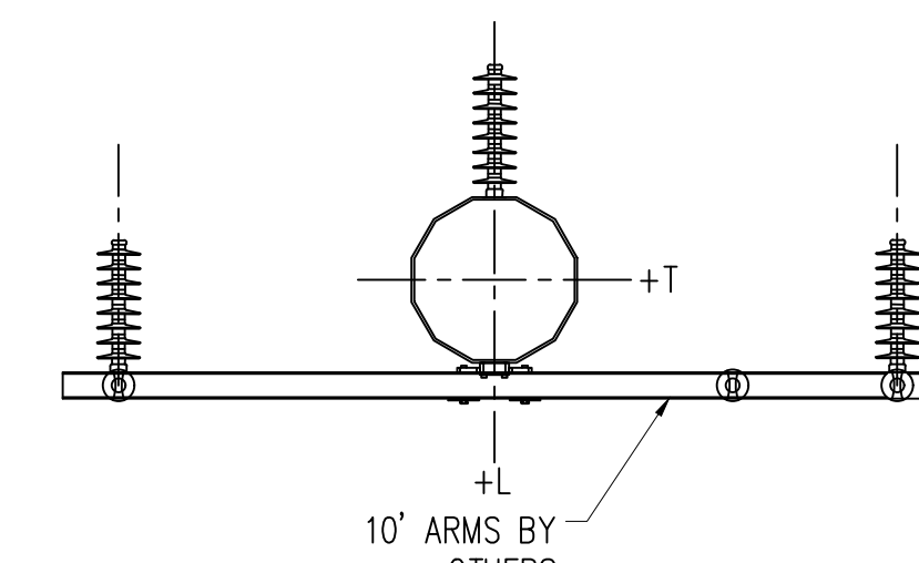
SECTION C-C (N.T.S.) DISTRIBUTION ATTACHMENT 795 KCMIL AAC "ARBUS" *DISTRIBUTION CENTRAL PHASE DEADEND INSULATOR ATTACHMENT AT TOP BOLT LOCATION OF CROSSARM MOUNT
