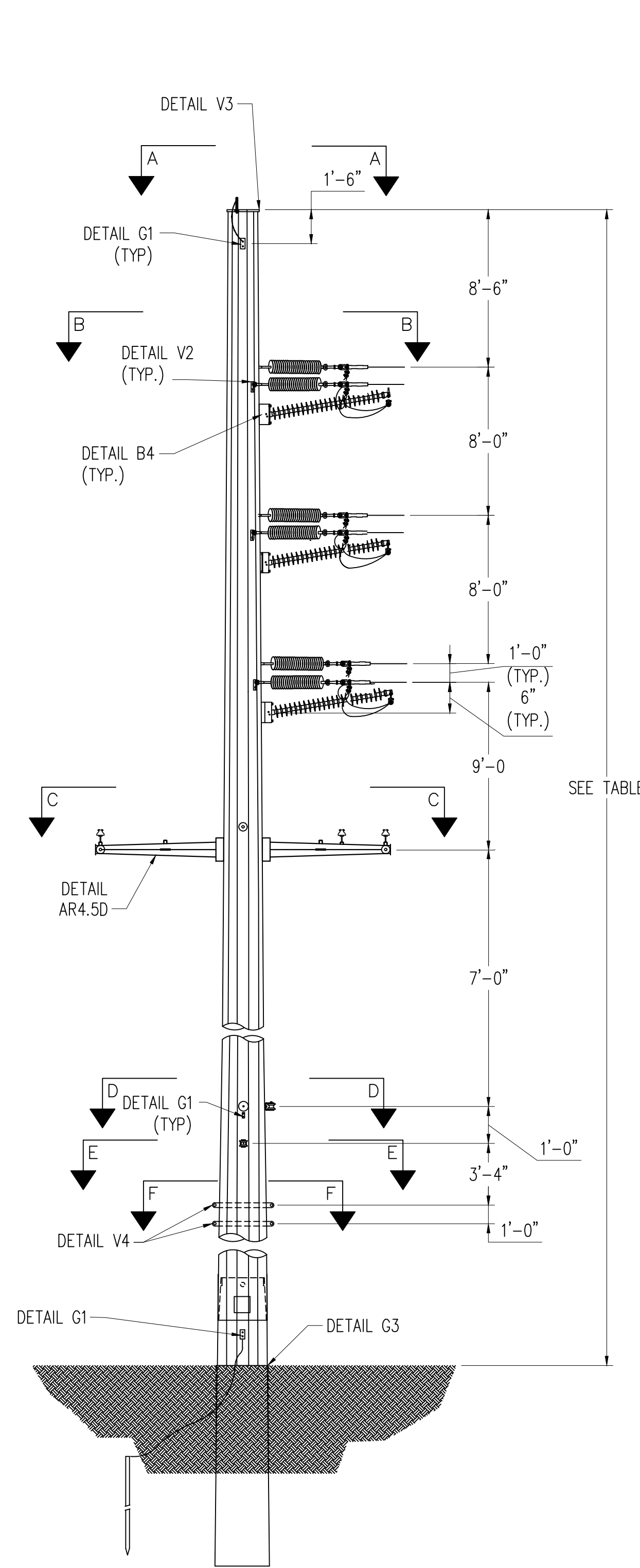
SINGLE CIRCUIT VERTICAL DEADEND LOOKING AHEAD SPAN SCALE: N.T.S.
