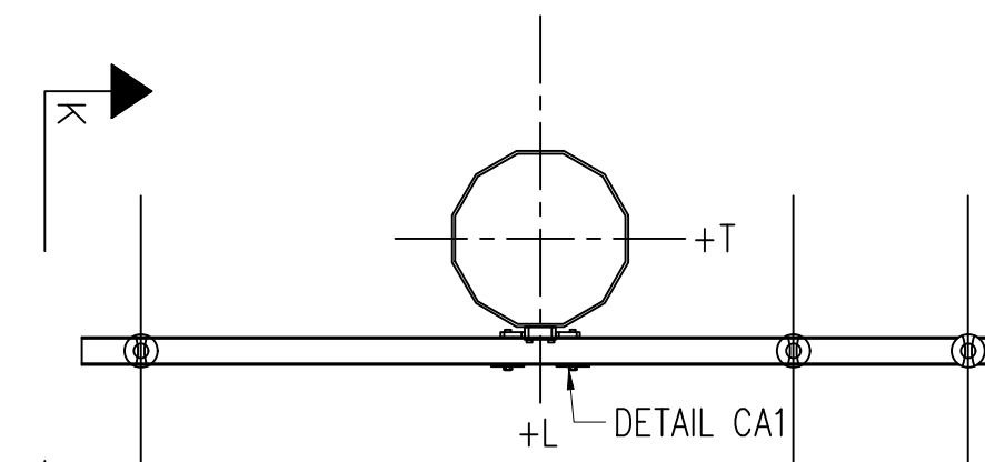
SECTION E-E (N.T.S.) DISTRIBUTION ATTACHMENT, 795 KCMIL AAC "ARBUTUS"
