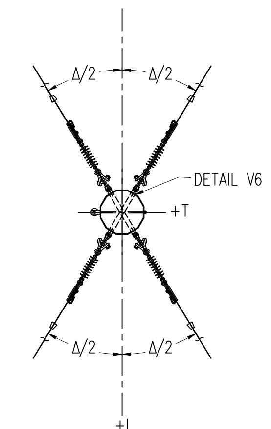
SECTION G-G (N.T.S.) NEUTRAL ATTACHMENT 336.4 KCMIL 18/1 STRAND "MERLIN" ACSR
