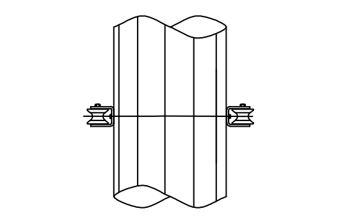
SECTION J-J (N.T.S.) COMMUNICATIONS ATTACHMENT "AT-XXX27DT-144-CLCB" 144 FIBER
