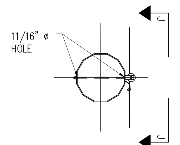
SECTION H-H (N.T.S.) COMMUNICATIONS ATTACHMENT ADSS: "AT-XXX27DT-144-CLCB" 144 FIBER
