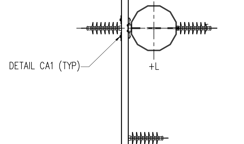
SECTION L-L (N.T.S.) DISTRIBUTION ATTACHMENT 1/0 AMG 6/1 STRAND "RAVEN" ACSR *DISTRIBUTION DEADEND NOTE
