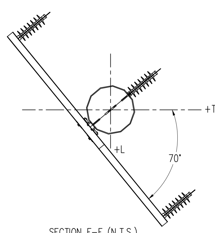
SECTION F-F (N.T.S.) DISTRIBUTION ATTACHMENT 336.4 KCMIL 18/1 STRAND "MERLIN" ACSR *DISTRIBUTION CENTRAL PHASE DEADEND INSULATOR ATTACHMENT AT TOP BOLT LOCATION OF CROSSARM MOUNT
