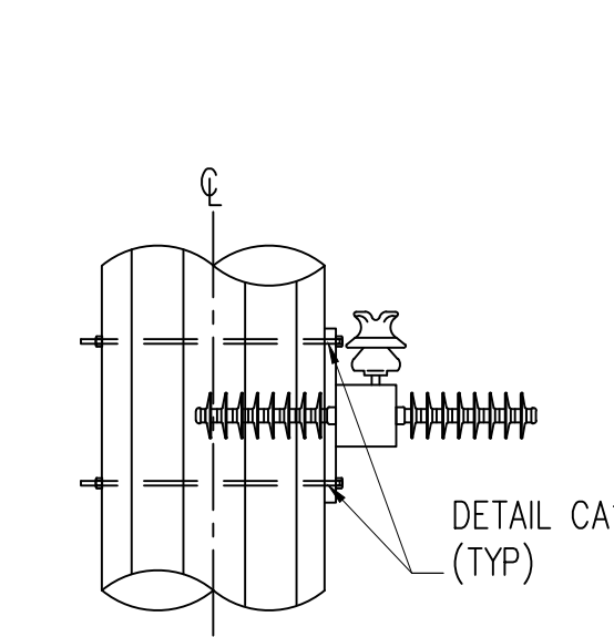
SECTION G-G (N.T.S.) DISTRIBUTION ATTACHMENT VARIOUS - SEE TABLE
