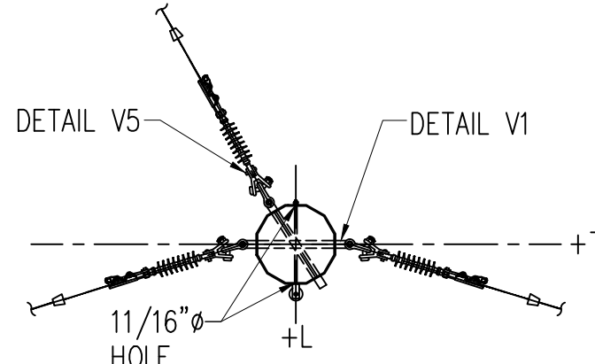
SECTION G-G (N.T.S.) DISTRIBUTION ATTACHMENTS 1/0 ACSR "RAVEN"
