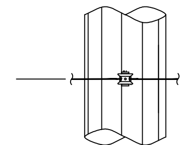
SECTION J-J (N.T.S.) COMMUNICATIONS ATTACHMENT ADSS: "AT-XXX27DT-144-CLCB" 144 FIBER
