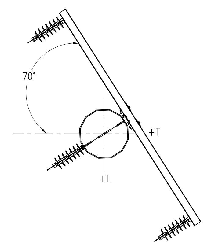
SECTION D-D (N.T.S.) DISTRIBUTION ATTACHMENT 795 KCMIL AAC "ARBUTUS" *DISTRIBUTION CENTRAL PHASE DEADEND INSULATOR ATTACHMENT AT TOP BOLT LOCATION OF CROSSARM MOUNT
