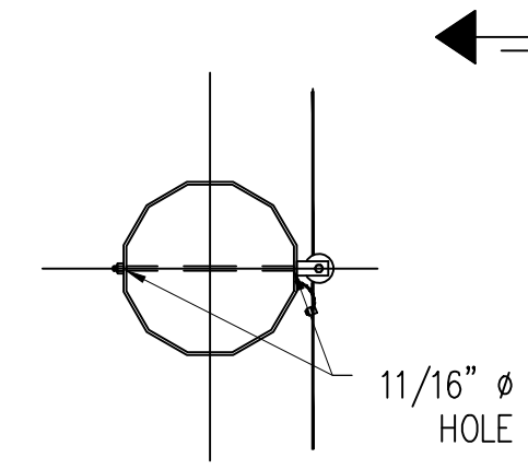
SECTION G-G (N.T.S.) DISTRIBUTION NEUTRAL 336.4 KCMIL 18/1 STRAND "MERLIN" ACSR
